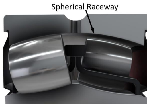
Spherical Roller Bearing Cross Section
