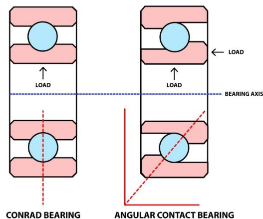
Bearing Comparison
